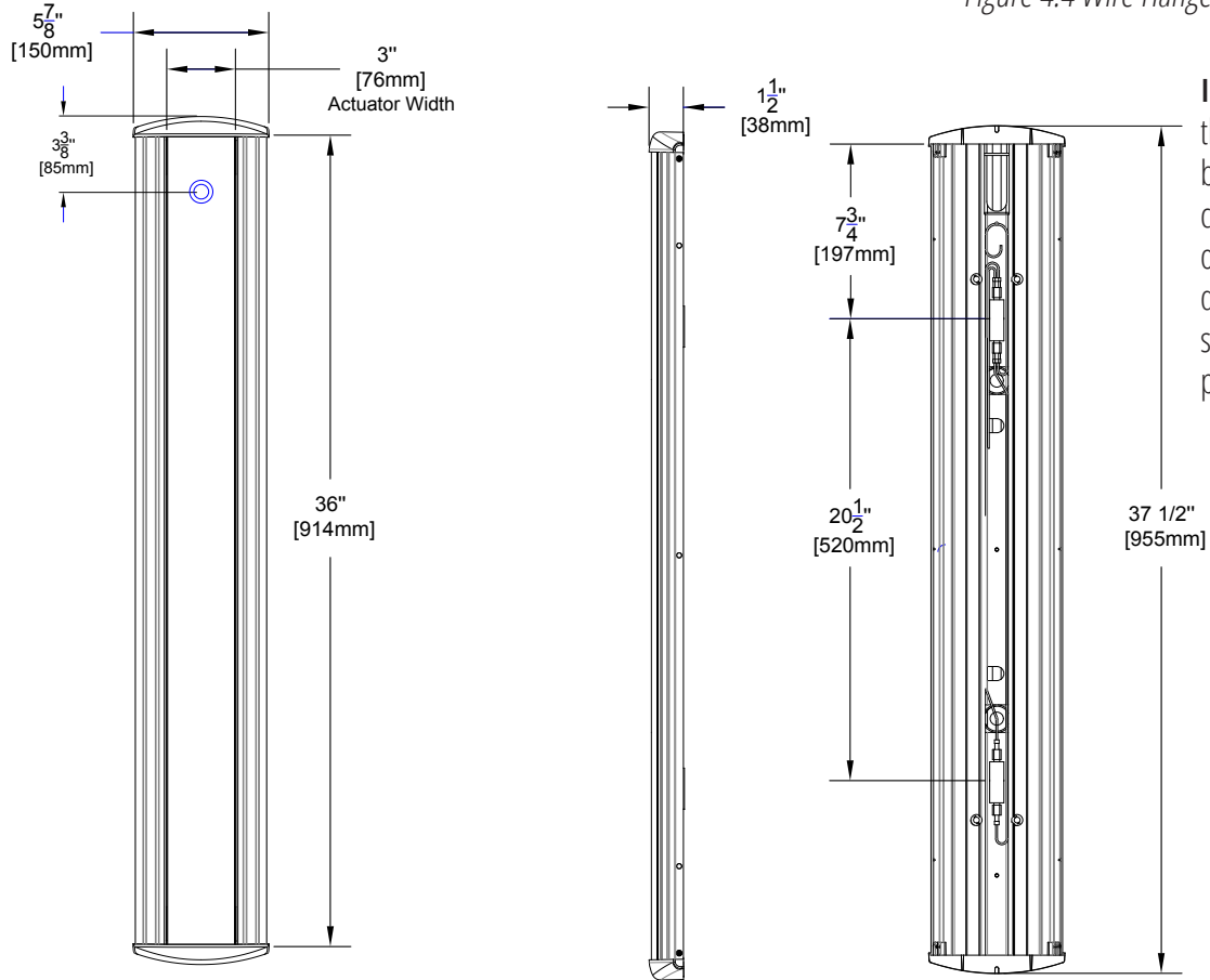
Figure 4.3 Dimensions
