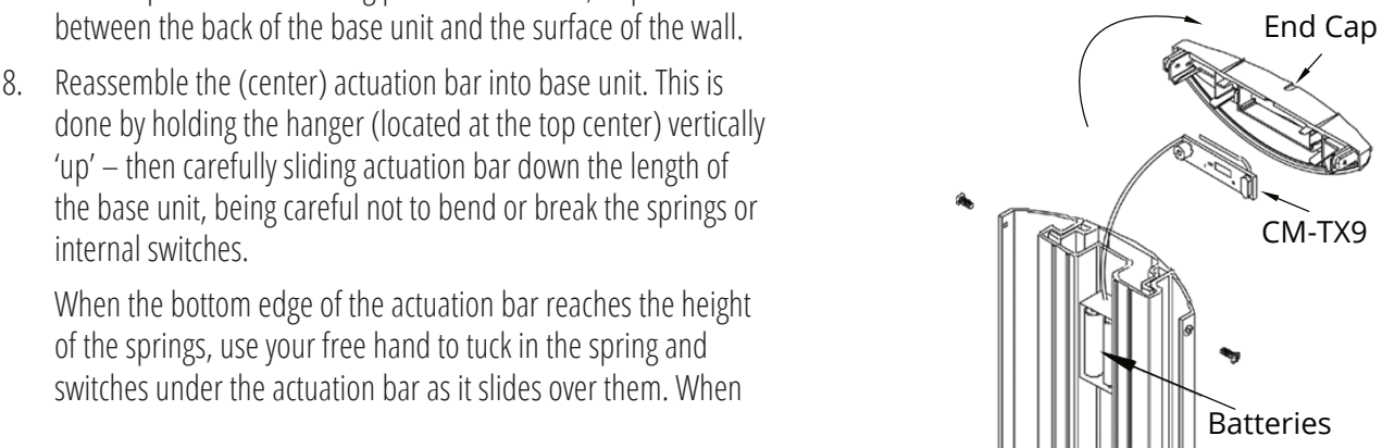
Figure 4.4 Wire Hanger/ End Cap
